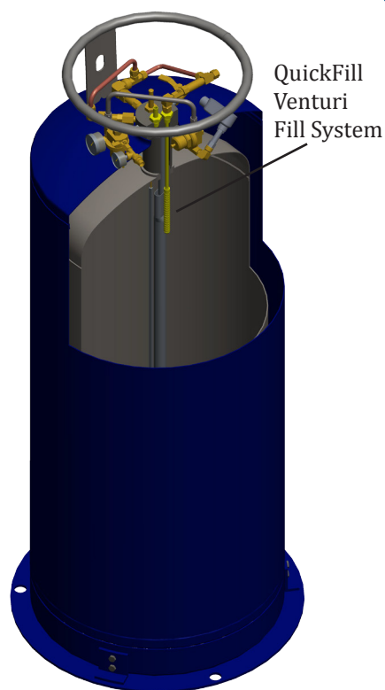
New Seismic Anchoring Tank Ring and QuickFill Venturi Fill System.
