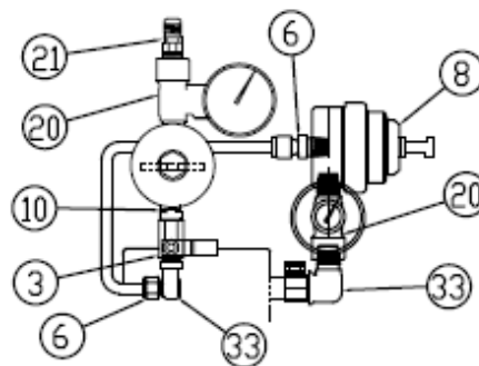
ECONOMIZER & GAS SUPPLY CIRCUIT
